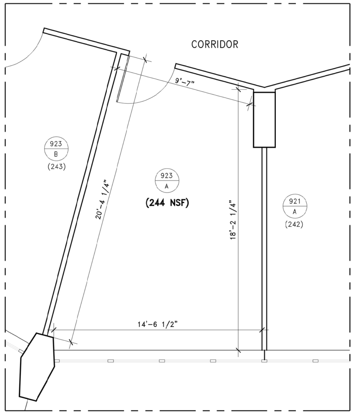
ULLMANN 9TH FLOOR PARTIAL PLAN SCALE: 1/4" = 1' - 0"
