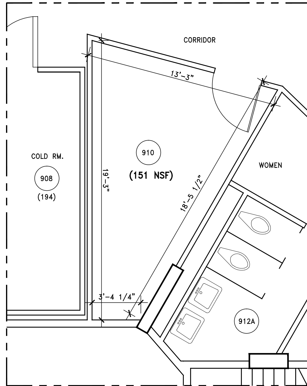
ULLMANN 9TH FLOOR PARTIAL PLAN SCALE: 1/4" = 1' - 0"
