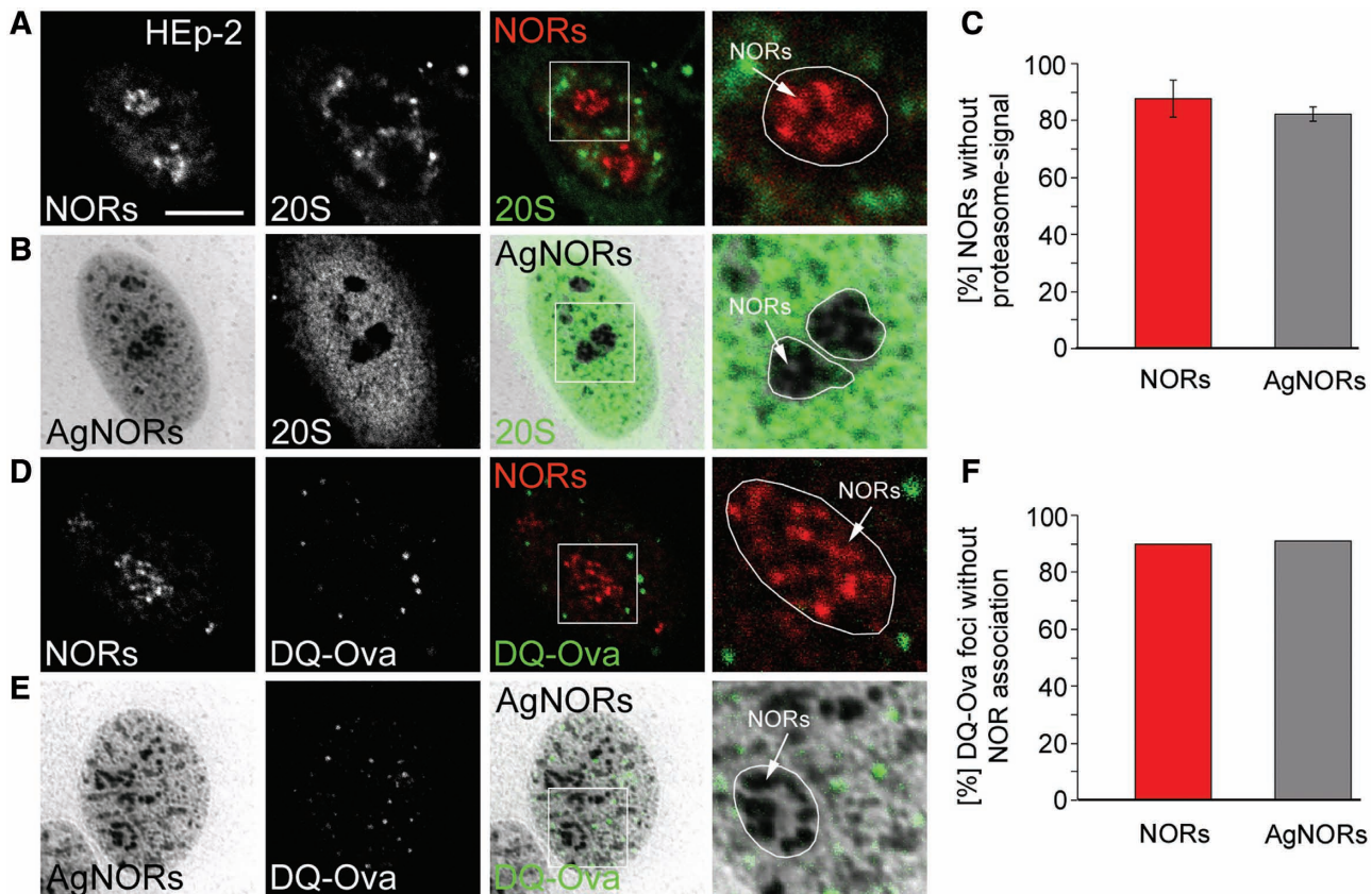
Figure 4. Proteasomes and proteasomal activity are not localized at sites of ribosomal RNA transcription. Endogenous gene array: ribosomal genes are labelled by a human patient serum against nucleolar organizer regions (NORs, A,D) or silverstaining (B and E). (A, B, D and E) Confocal fluorescence micrographs of NORs in representative HEP-2 cells double-labelled with antibodies against proteasomes (green; A and B) or micro-injected with DQ-Ova (green; D, E). Bar, 5 \mu m. Quantification of (C) NORs in relation to proteasomes from three independent experiments ( n = 300 ) and (F) the positioning of proteolytic foci in relation to NORs from three independent experiments (NORs: n = 19 ; AgNORs: n = 22 ).
